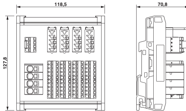
Dimensioned drawing
