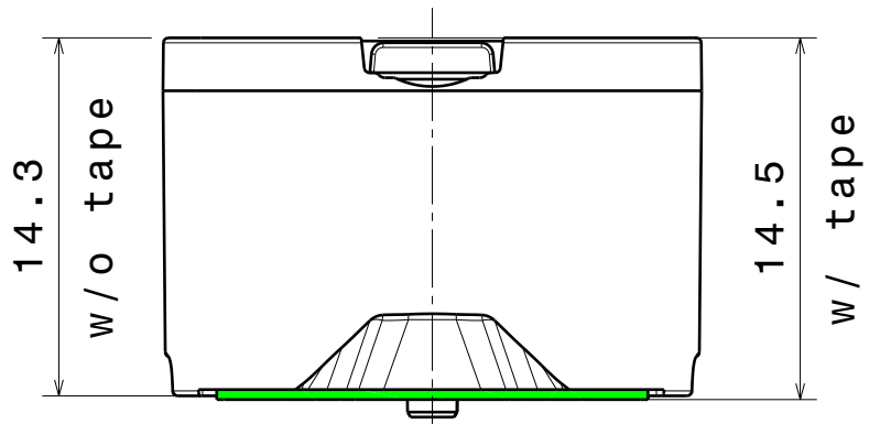
Front view Scale: 3:1
