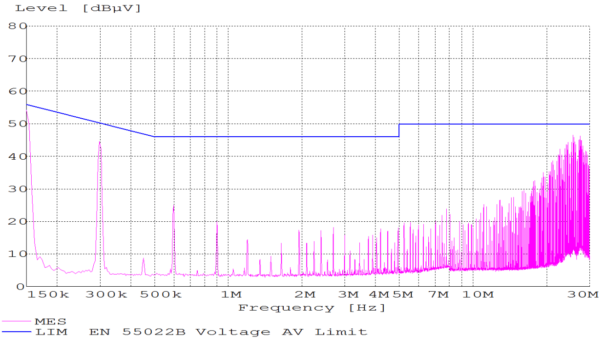
Figure 23. EMC Considerations
