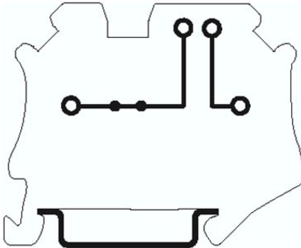
Circuit diagram
