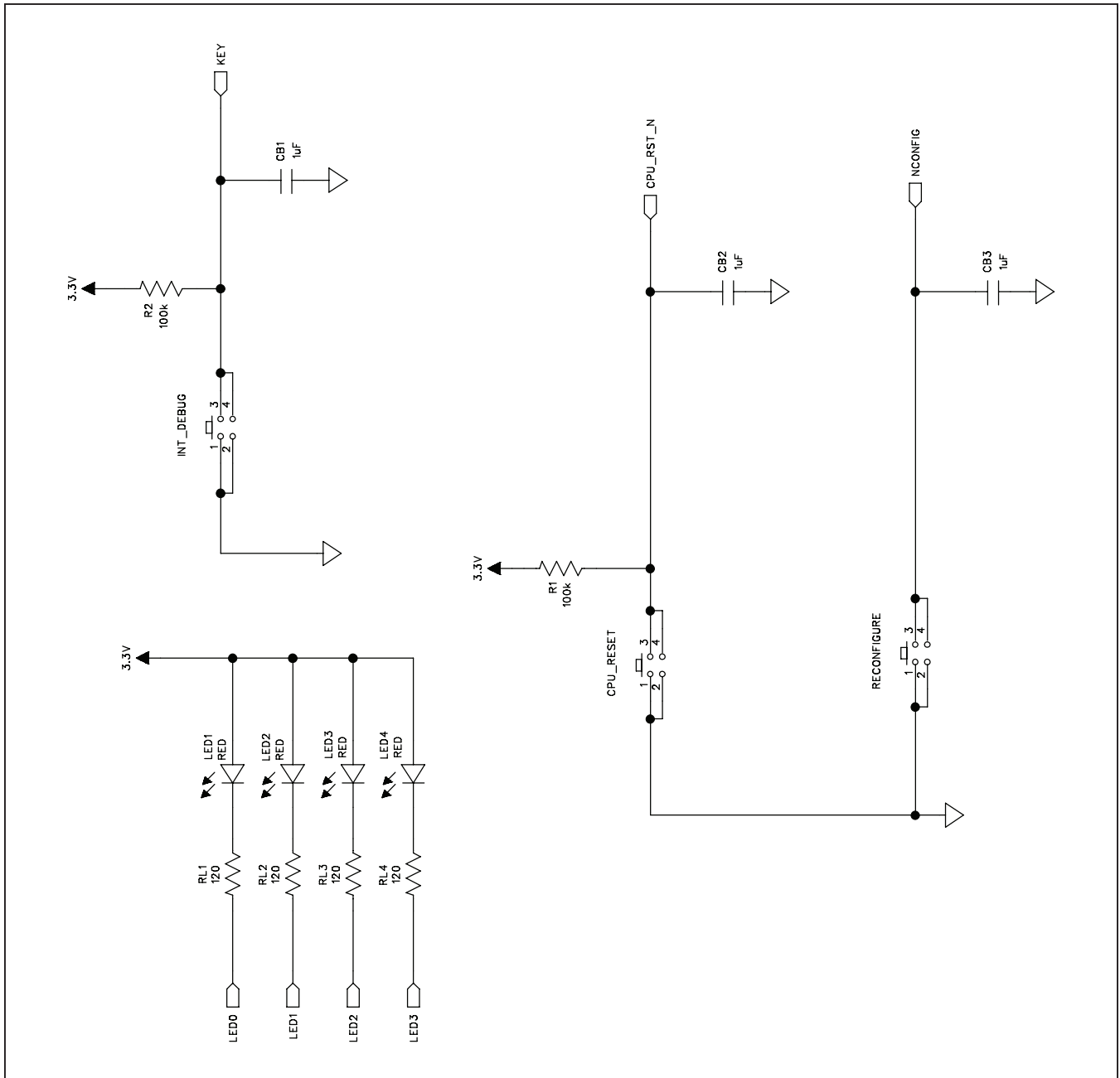
Figure 8i. MAX1131 EV Kit Schematic (Sheet 9 of 14)
