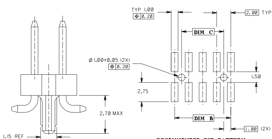
RECOMMENDED PCB PATTERN (SCALE 5 : 1)
