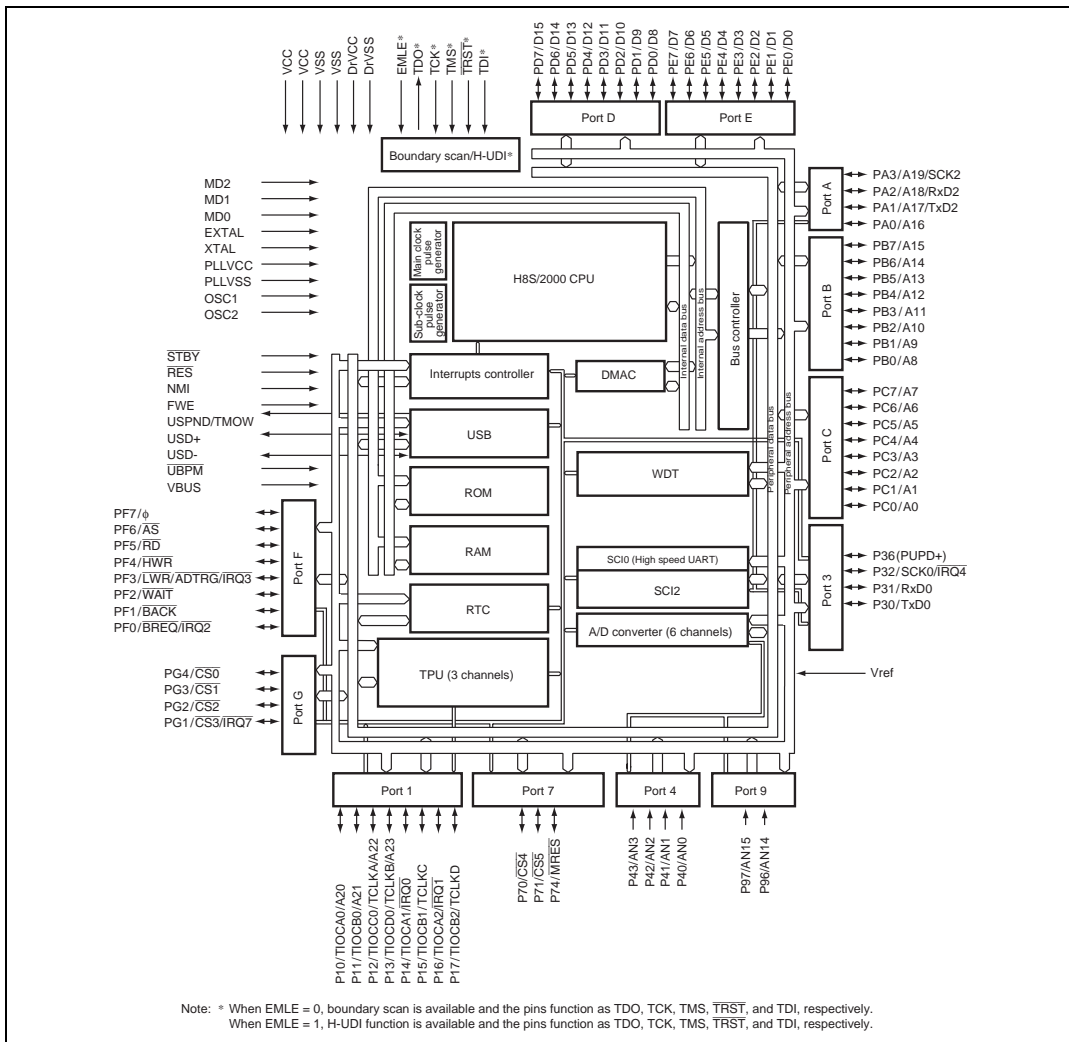
Figure 1.1 Internal Block Diagram of HD64F2218, HD64F2218U, HD64F2218CU and HD642217CU
