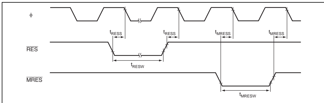
Figure 22.5 Reset Input Timing
