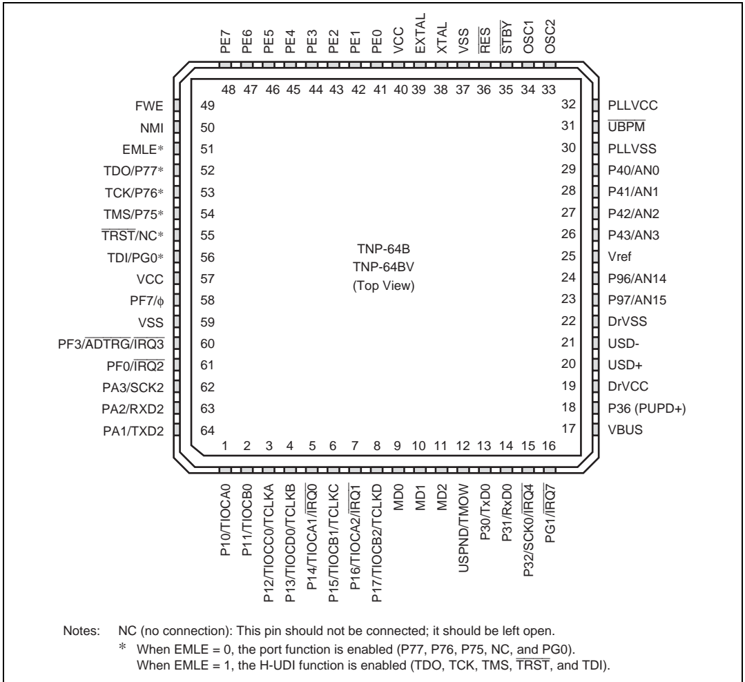
Figure 1.11 Pin Arrangements of HD64F2212, HD64F2212U, HD64F2212CU, HD64F2211, HD64F2211U, HD64F2211CU and HD64F2210CU (TNP-64B, TNP-64BV)
