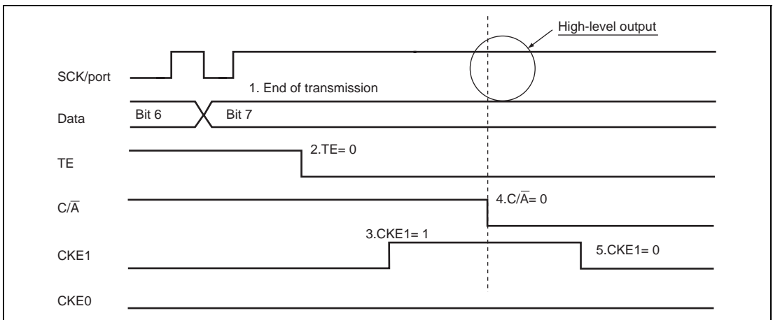
Figure 12.44 Operation when Switching from SCK Pin Function to Port Pin Function (Example of Preventing Low-Level Output)
