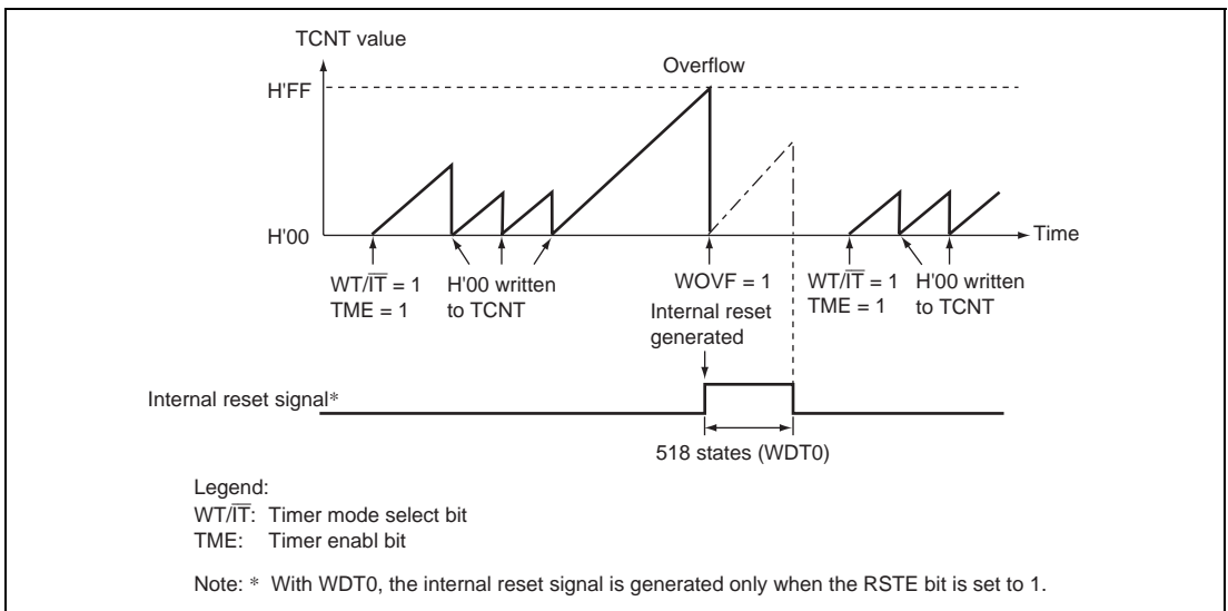
Figure 10.2 Operation in Watchdog Timer Mode
