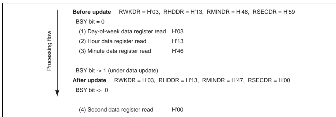
Figure 11.4 Example: Reading of Inaccurate Time Data
