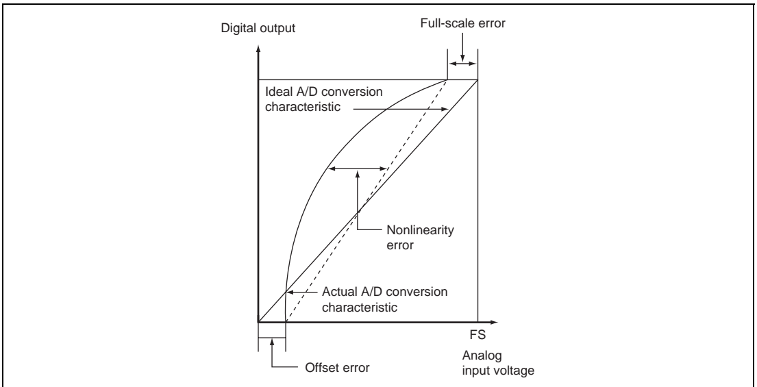
Figure 15.8 A/D Conversion Precision Definitions (2)
