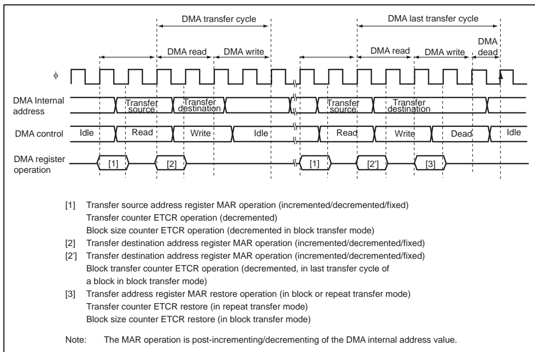
Figure 7.25 DMAC Register Update Timing
