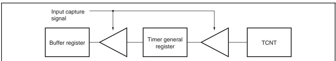
Figure 9.17 Input Capture Buffer Operation
