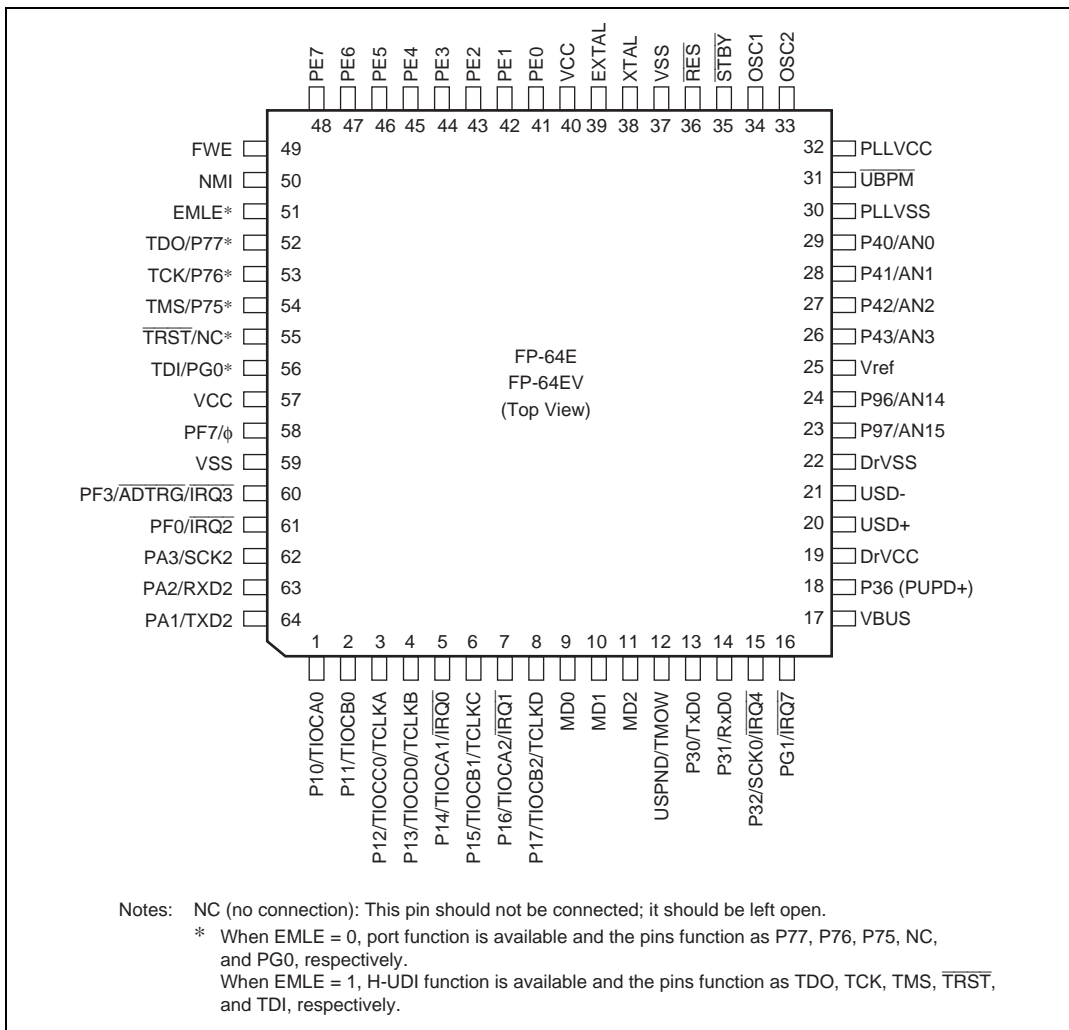
Figure 1.9 Pin Arrangements of HD64F2212, HD64F2212U, HD64F2212CU, HD64F2211, HD64F2211U, HD64F2211CU and HD64F2210CU (FP-64E, FP-64EV)
