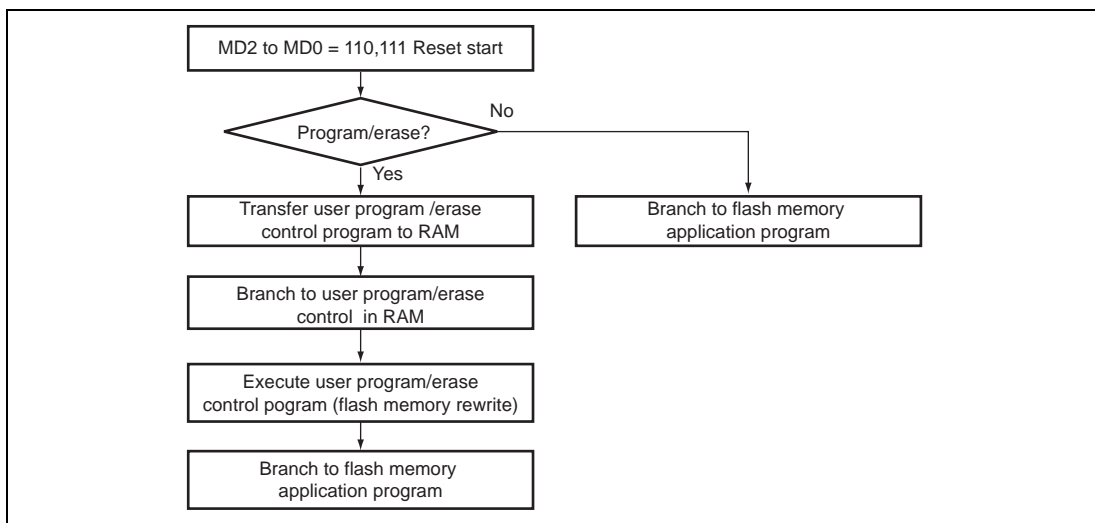
Figure 17.10 Programming/Erasing Flowchart Example in User Program Mode
