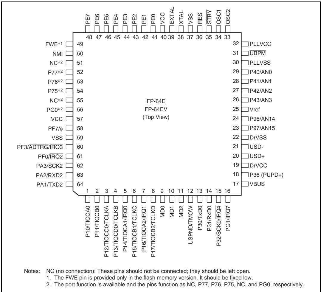
Figure 1.10 Pin Arrangements of HD6432211, HD6432210 and HD6432210S (FP-64E, FP-64EV)
