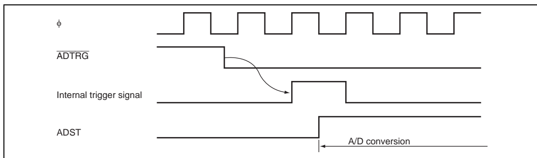
Figure 15.6 External Trigger Input Timing
