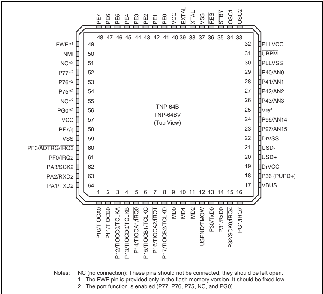
Figure 1.12 Pin Arrangements of HD6432211, HD6432210 and HD6432210S (TNP-64B, TNP-64BV)
