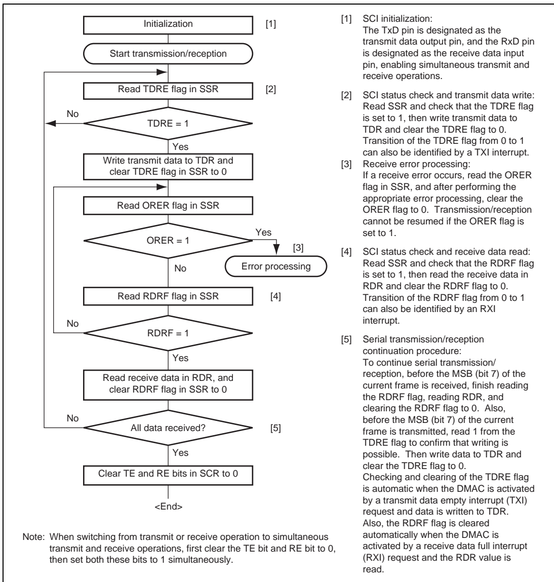
Figure 12.23 Sample Flowchart of Simultaneous Serial Data Transmit and Receive Operations
