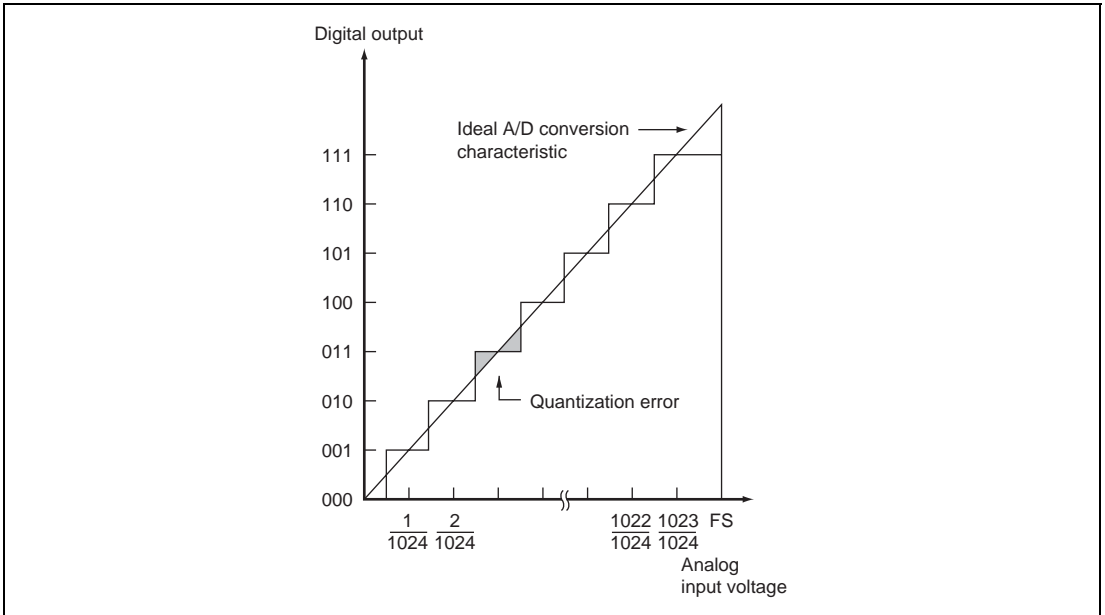
Figure 15.7 A/D Conversion Precision Definitions (1)
