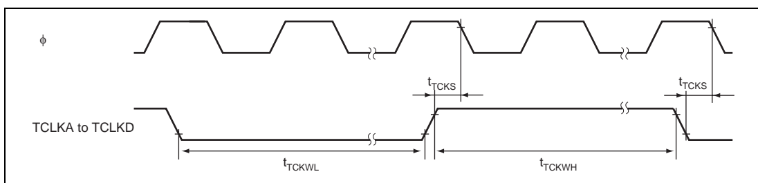
Figure 22.14 TPU Clock Input Timing
