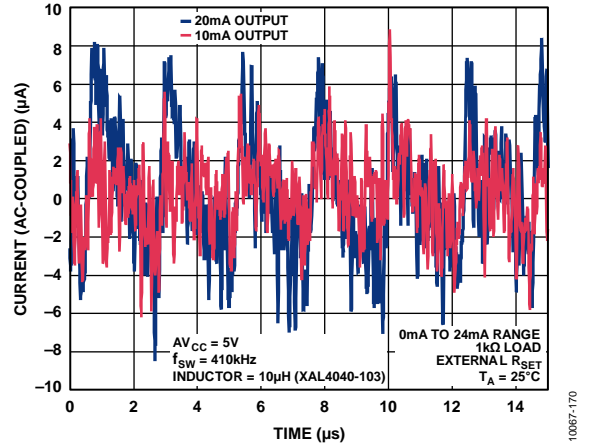
Figure 30. Output Current, AC-Coupled vs. Time with DC-to-DC Converter (See Figure 56)
