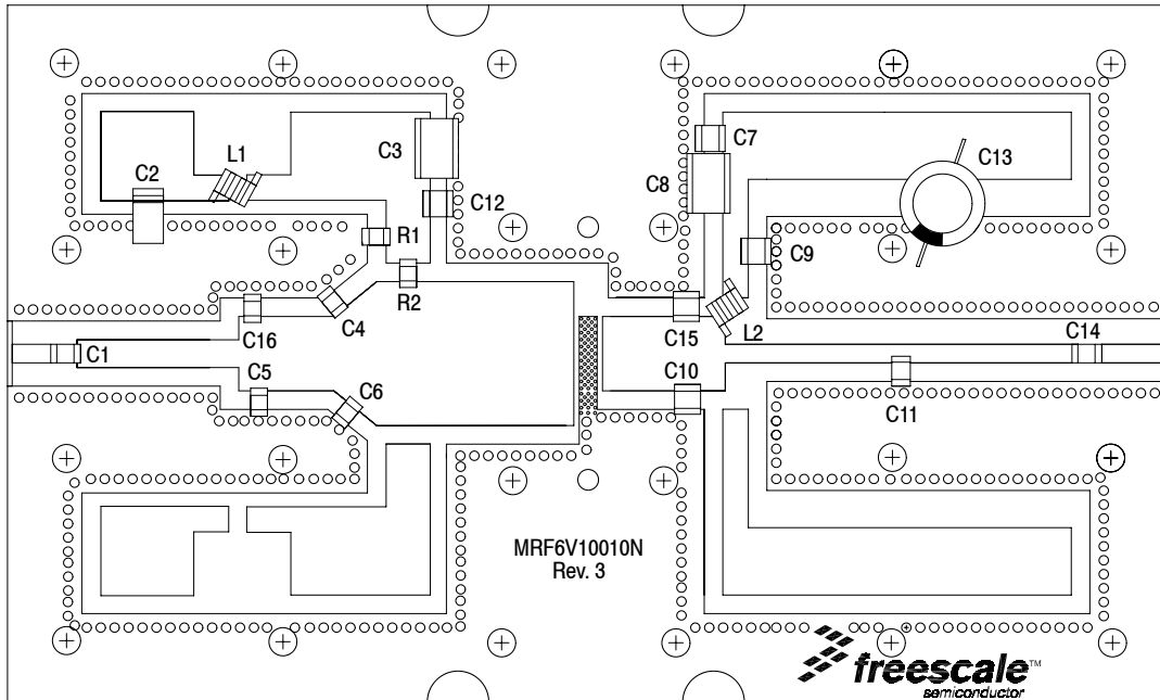
Figure 2. MRF6V1001NR4 Test Circuit Component Layout
