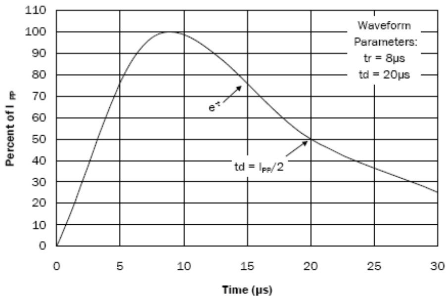
Fig.2 Pulse Waveform
