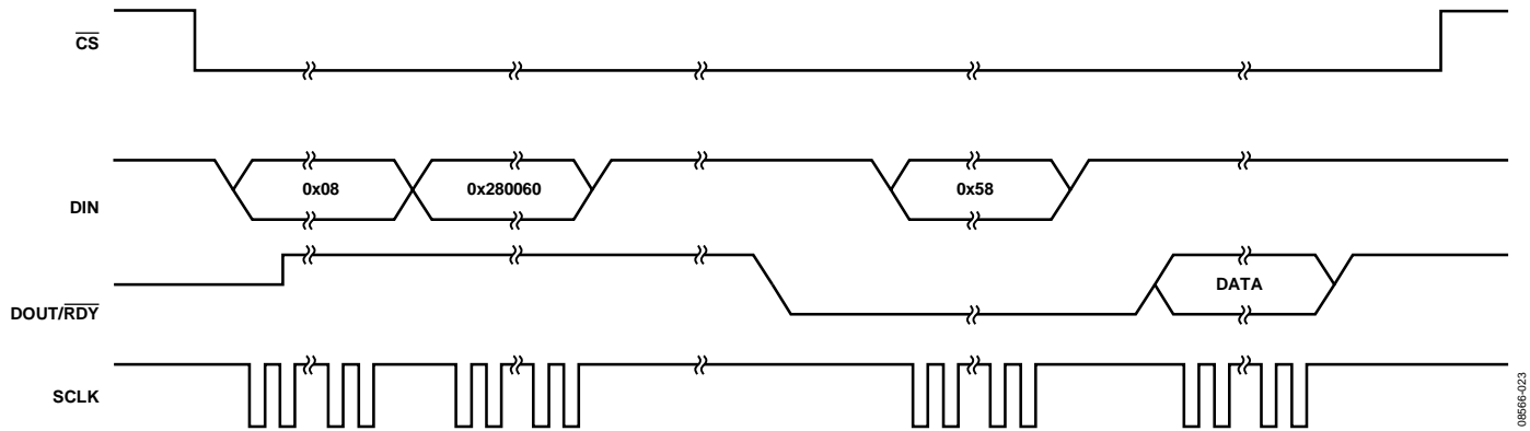
Figure 24. Single Conversion
